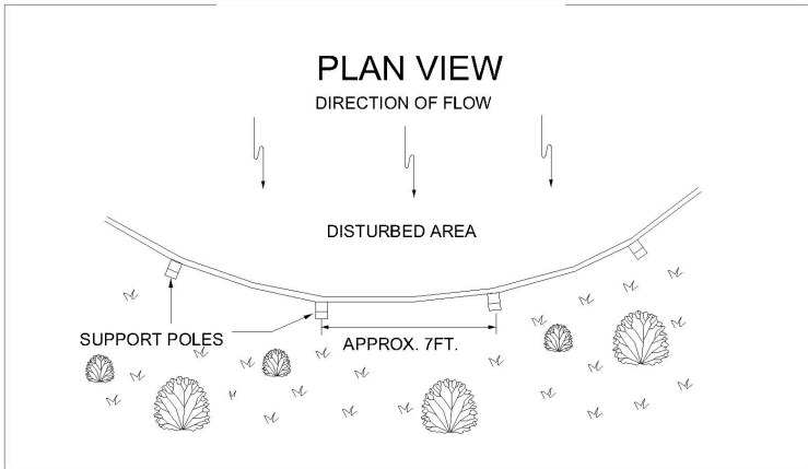
Figure 9. Silt Fence
